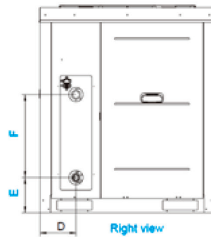
Right view MC-SU30-RN1L / MC-SU60-RN1L
